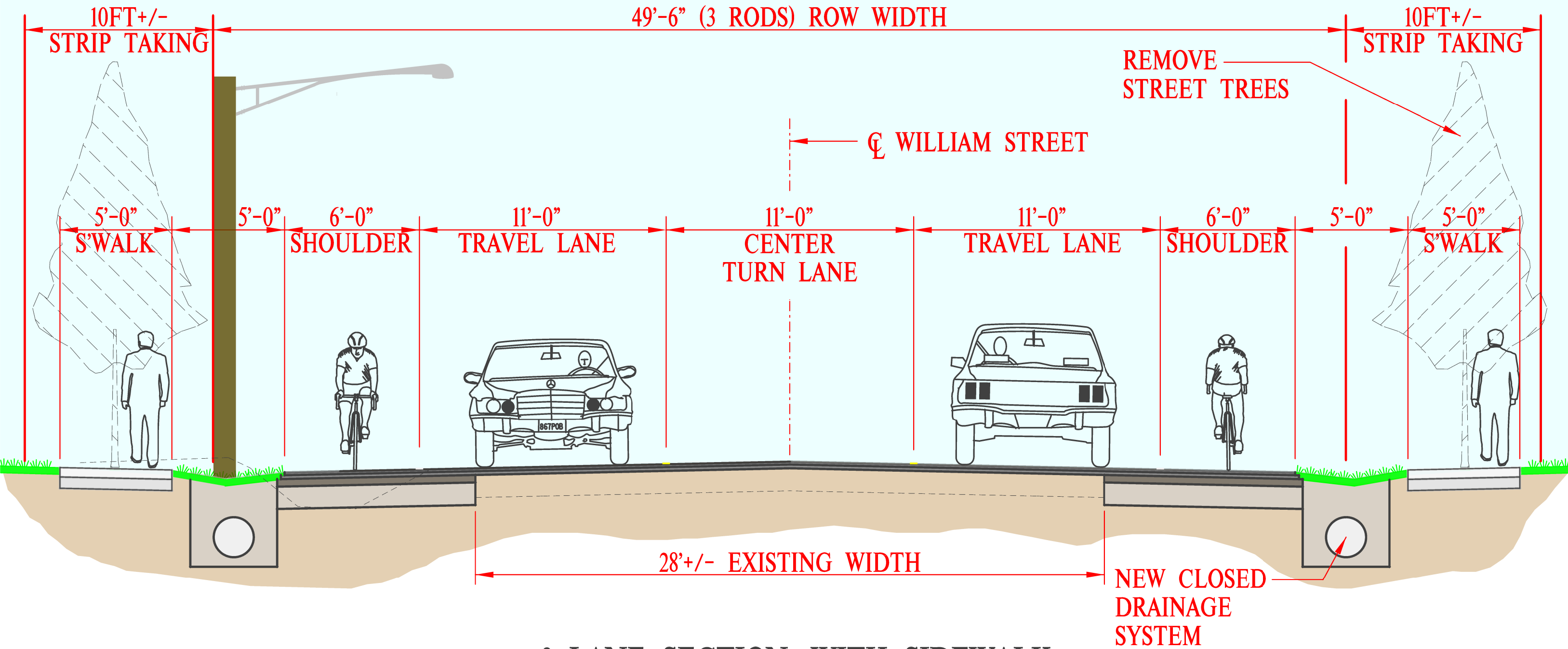
3 LANE SECTION, WITH SIDEWALK
