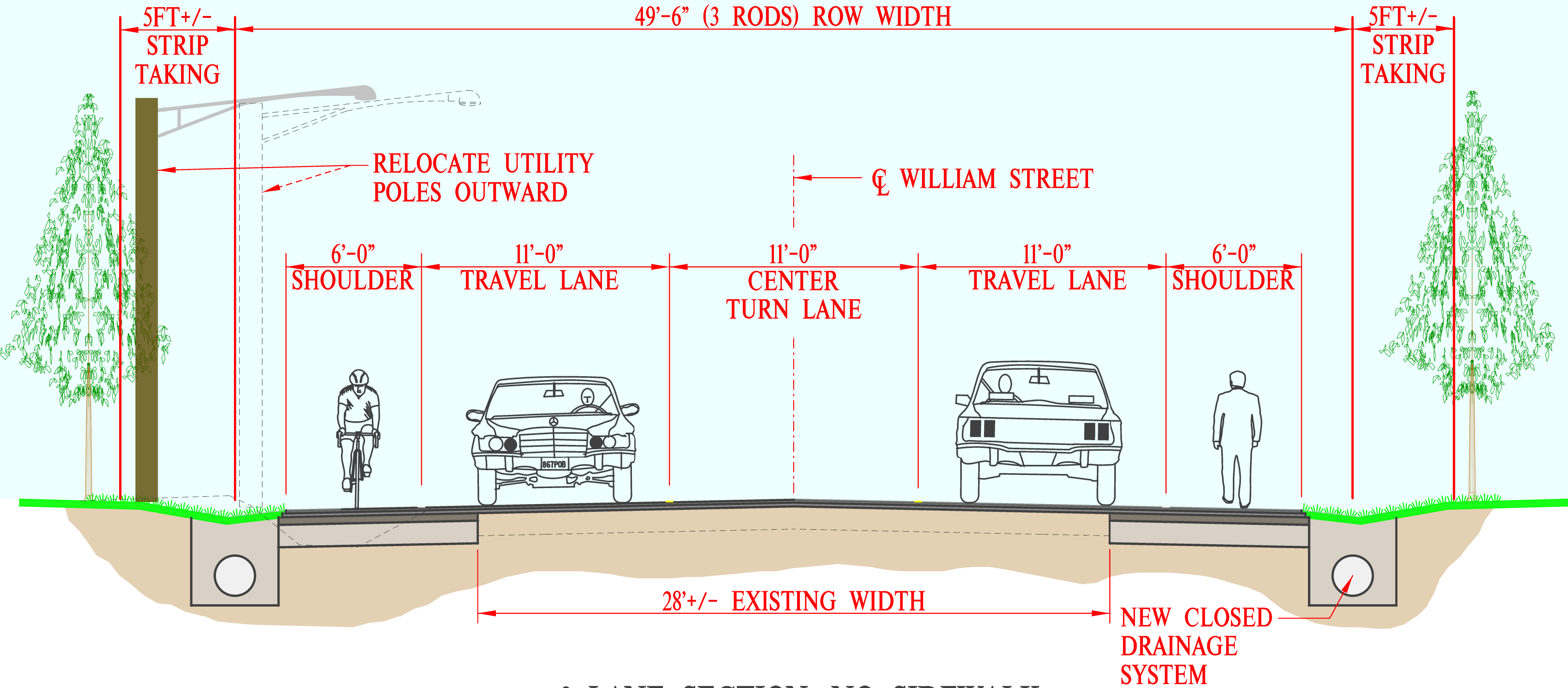
3 LANE SECTION, NO SIDEWALK
