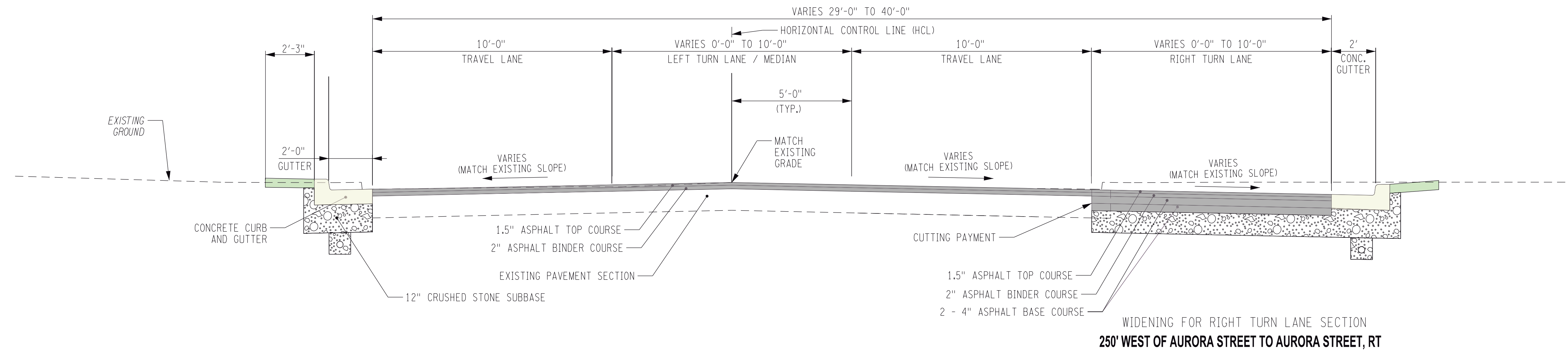
AURORA STREET TWO COURSE MILL AND OVERLAY WITH WIDENING FOR RIGHT TURN LANE NOT TO SCALE
